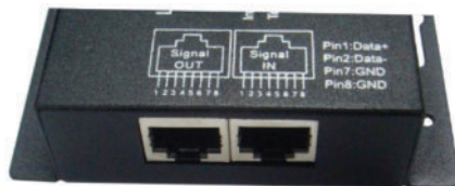
RJ45 network cable ports
