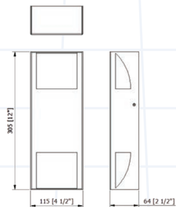
WING TLWMMV15XWMZZ-02
