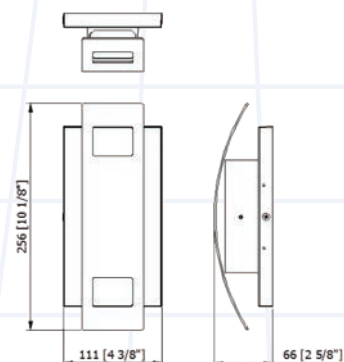
WAVE TLWMMV15XWMZZ-01
