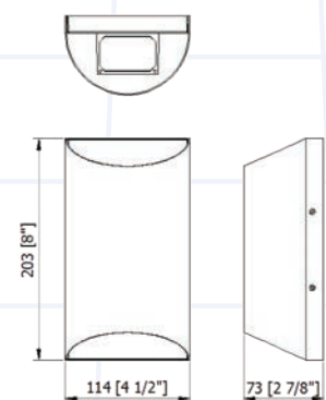
SCOOP TLWMMV15XWMZZ-04
