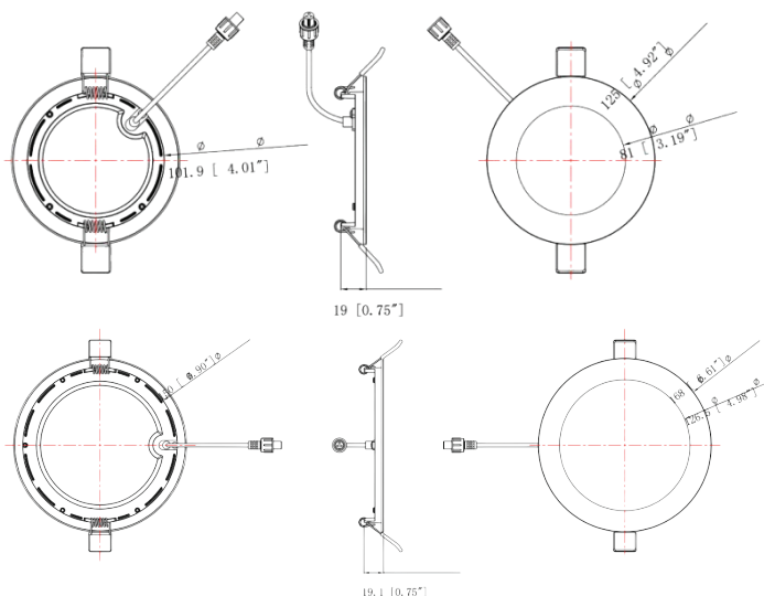
Dimensions for 6-inch: Cut-out size: 6.375"
